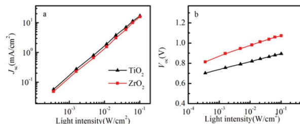
Fig. 4 The light intensity dependence of J_{sc} (a) and V_{oc} (b) in spiro-OMeTAD/ \text{CH}_3\text{NH}_3\text{PbI}_3/\text{ZrO}_2 (or \text{TiO}_2 ) solar cells.
