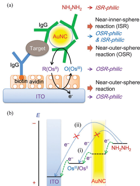
Fig. 1 (a) Schematic of an immunosensor using outer-sphere to inner-sphere electrochemical-nanocatalytic ( EN_c ) redox cycling. (b) Schematic of three-step electron transfer related to EN_c redox cycling (green lines) and unwanted electron transfer (sky-blue lines). The applied potential, the formal potentials of Os^{III}(bpy)_2Cl_2^+/Os^{II}(bpy)_2Cl_2 and hydrazine, and the potential of the Au nanocatalyst (AuNC) (horizontal lines) are positioned in order of potential.
