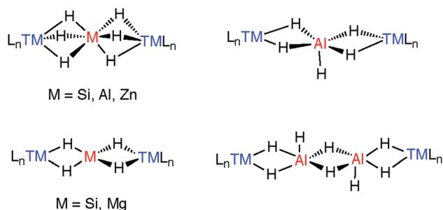
Fig. 22 Coordination geometries of trapped \text{MH}_x units and comparison to silane chemistry.
