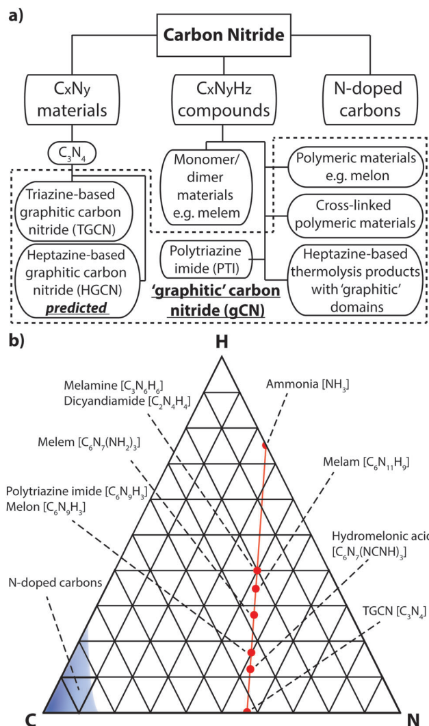
Fig. 2 (a) Diagram showing the various classes of carbon nitrides. The dashed box indicates materials often designated graphitic carbon nitride (gCN). (b) Ternary plot of important types of carbon nitride materials projected on to a C–N–H compositional diagram. Semimetallic N-doped graphite and graphene materials cluster near the pure C pole (elemental analysis results based on ref. 29 and 30), whereas stoichiometric gCN compounds are concentrated around a tie-line extending between melamine or DCDA to approximately C 2 N 3 H via loss of NH 3 component. Complete loss of NH 3 would result in C 3 N 4 .
