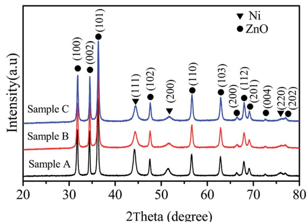
Fig. 1 XRD patterns of the Ni/ZnO composites prepared with different solvent solutions.
