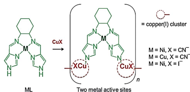
Scheme 3 Synthesis of [\text{NiL}]_2[\text{Cu(I)CN}]_9_n , [\text{Cu(II)L}]_2[\text{Cu(I)CN}]_9_n and [\text{NiL}][\text{Cu(II)I}]_2_n . [Reproduced from ref. 101 with permission from The Royal Society of Chemistry.]
