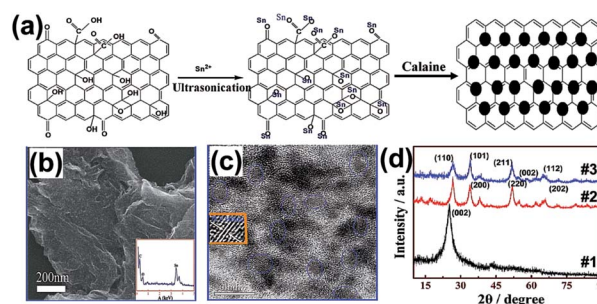
Fig. 10 (a) Schematic diagram of the formation of a SnO 2 QDs/GR hybrid. (b) Field emission-secondary electron microscopy (FE-SEM) image of the SnO 2 QDs/GR hybrid on the Si (100) substrate. (c) HRTEM image of the SnO 2 QDs/GR hybrid. (d) XRD patterns of bare graphene sheets (#1), SnO 2 QDs/GR hybrid (#2) and SnO 2 nanoparticles (#3). Reprinted with permission from ref. 68. Copyright 2013 American Chemical Society.
