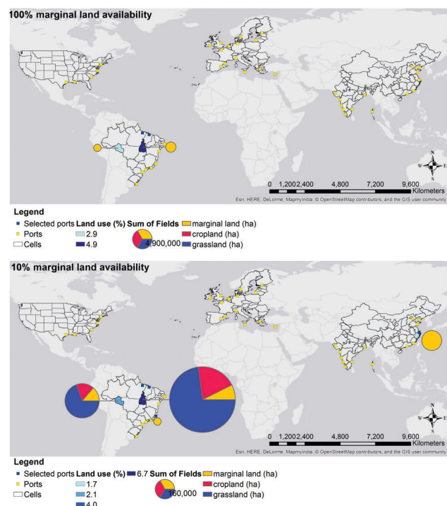
Fig. 7 Evolution of BECCS optimal value chain in the water minimisation scenario at 0% AR availability, and constraining marginal land availability from 100% to 10%.
