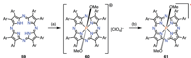
Fig. 19 Synthesis of 61 . (a) POBr_3 (200 equiv.), pyridine, 90^\circ C , 15 h, then CH_2Cl_2/MeOH , rt, 1 d. 60 was separated by SiO_2 column chromatography ( CH_2Cl_2/MeOH/CF_3CO_2H = 90/9.5/0.5 ), then NaClO_4 , CH_2Cl_2/MeCN , rt, 12 h, 56%; (b) 61 was separated by Al_2O_3 column chromatography (eluent: CH_2Cl_2/TEA = 99.5/0.5 ) without isolating 60 , 44%.
