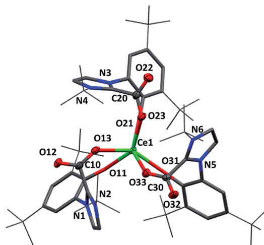
Fig. 2 Molecular structures of 2\text{Ce}^{i\text{Pr}} (upper) and 2\text{Ce}^{t\text{Bu}} (lower) with carboxylate and Ce atoms shown at 50% ellipsoid probability, framework and peripheral carbon atoms drawn capped stick and wireframe respectively, and H and lattice solvent omitted for clarity. Selected distances (Å) and angles ( ^\circ ) for 2\text{Ce}^{i\text{Pr}} : Ce1–O11 2.790(5), Ce1–O21 2.274(5), Ce1–O31 2.256(6), Ce1–O13 2.468(6), Ce1–O23 2.482(6), Ce1–O33 2.466(6), O11–Ce1–O21 97.18(19), O11–Ce1–O31 99.3(2), O21–Ce1–O31 94.8(2), O13–Ce1–O23 77.02(19), O13–Ce1–O33 76.68(19), O23–Ce1–O33 79.6(2), O11–Ce1–O13 75.72(19), O21–Ce1–O23 75.7(2), O31–Ce1–O33 75.9(2). For 2\text{Ce}^{t\text{Bu}} : Ce1–O11 2.261(2), Ce1–O21 2.268(2), Ce1–O31 2.274(2), Ce1–O13 2.473(2), Ce1–O23 2.477(2), Ce1–O33 2.470(2), O11–Ce1–O21 95.38(8), O11–Ce1–O31 95.25(8), O21–Ce1–O31 97.20(8), O13–Ce1–O23 76.76(8), O13–Ce1–O33 80.89(8), O23–Ce1–O33 80.80(8), O11–Ce1–O13 75.50(8), O21–Ce1–O23 74.77(2), O31–Ce1–O33 75.03(8).
