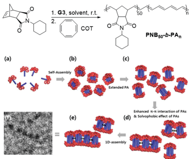
Fig. 1 Preparation of PNB 50 -b-PA n diblock copolymer “nanocaterpillars” via a one-pot ROMPISA process and proposed 1D self-assembly mechanism. Adapted with permission from ref. 37. Copyright 2012 American Chemical Society.
