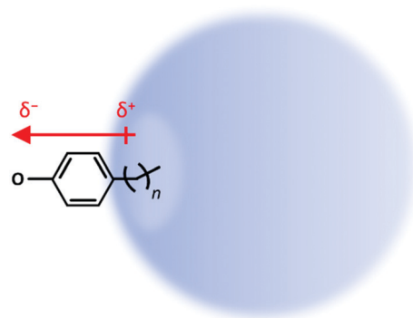
Fig. 1 Picture of dipole-bound state (DBS) of para -substituted alkylphenolate with varying chain length, n - ph^- .
