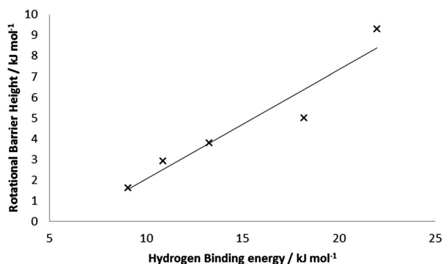
Fig. 8 Correlation between average HBE and average rotational barrier for 5 \text{H}_2 bound to \text{Mn}_5\text{H}_n ( n = 6-10 ).
