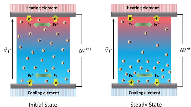
Fig. 1 Schematic images of an open-circuit thermocell containing redox molecules ( e.g. , Fc^+ (ferrocenium)/ Fc (ferrocene)) and charged nanoparticles. Left panel: Initial state immediately after the application of a temperature gradient where NP concentration is still homogeneous. Right panel: Steady state established after the completion of thermodiffusive movements of all charged species. Note that in the open-circuit configuration, there is no electric current flowing into and from the thermocell. Therefore both reduction and oxidation reactions occur at the hot and cold electrodes. In this example, the charged NPs move toward the cold region of the fluid, corresponding to a positive S_T . See the text for more explanation.
