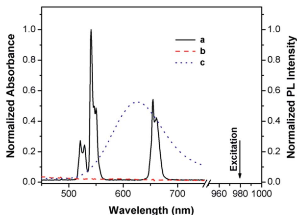
Fig. 2 UCL spectrum of DSPE-coated \text{NaYF}_4\text{:}20\%\text{Yb},2\%\text{Er} (DSPE-UCNPs) under excitation from a 980 nm laser (a), and UV-vis spectra of the protein apo-azurin in the absence (b) and presence of \text{Cu}^{2+} (c).
