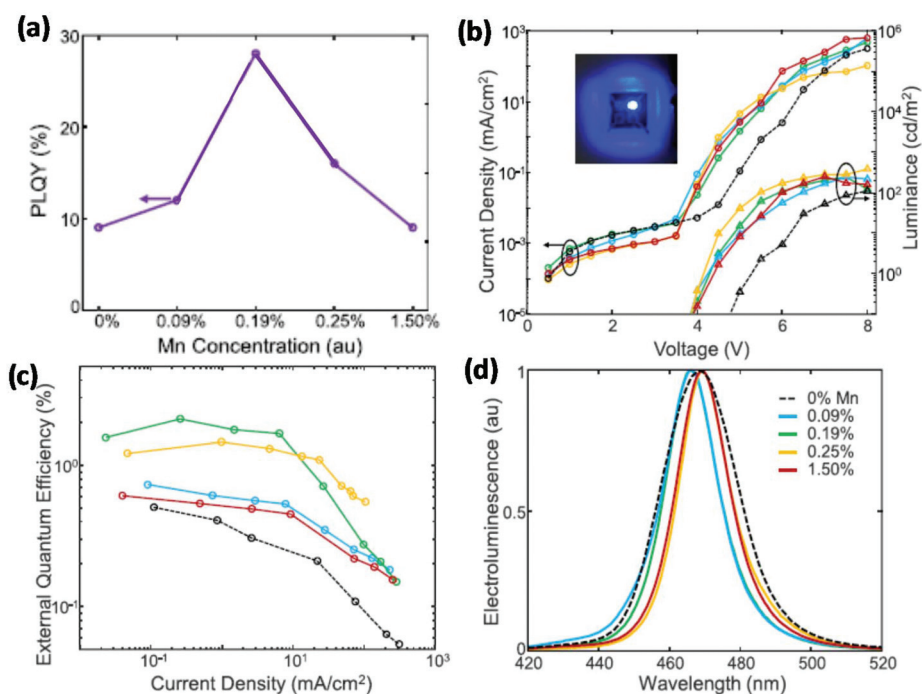
Fig. 5 Blue PeLEDs based on Mn-doped PNCs with various doping concentrations. (a) PLQEs of Mn-doped PNCs. (b) J-V-L characteristics; the inset image is a photograph of a blue LED under operation. (c) EQE-current density plots. (d) EL spectra. Reproduced with permission. 57 Copyright © 2018 Elsevier Inc.
