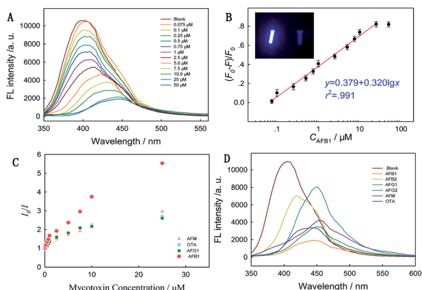
Fig. 3 Emission spectra of Zr-CAU-24 with the incremental addition of AFB1 in water, with toxin concentrations given from 0 to 50 \mu\text{M} (A). Linear relationship between \lg C_{\text{AFB1}} and FL intensity. Inset: optical photo of fluorescent Zr-CAU-24 crystals in water (left) and water (right) (B). Stern–Volmer curves acquired at \lambda_{\text{ex}} = 340 nm and \lambda_{\text{em}} = 410 nm for AFB1, AFG1, AFM and OTA (C). FL intensity fading of Zr-CAU-24 towards 50 \mu\text{M} AFB1, AFB2, AFG1, AFG2, AFM and OTA (D).
