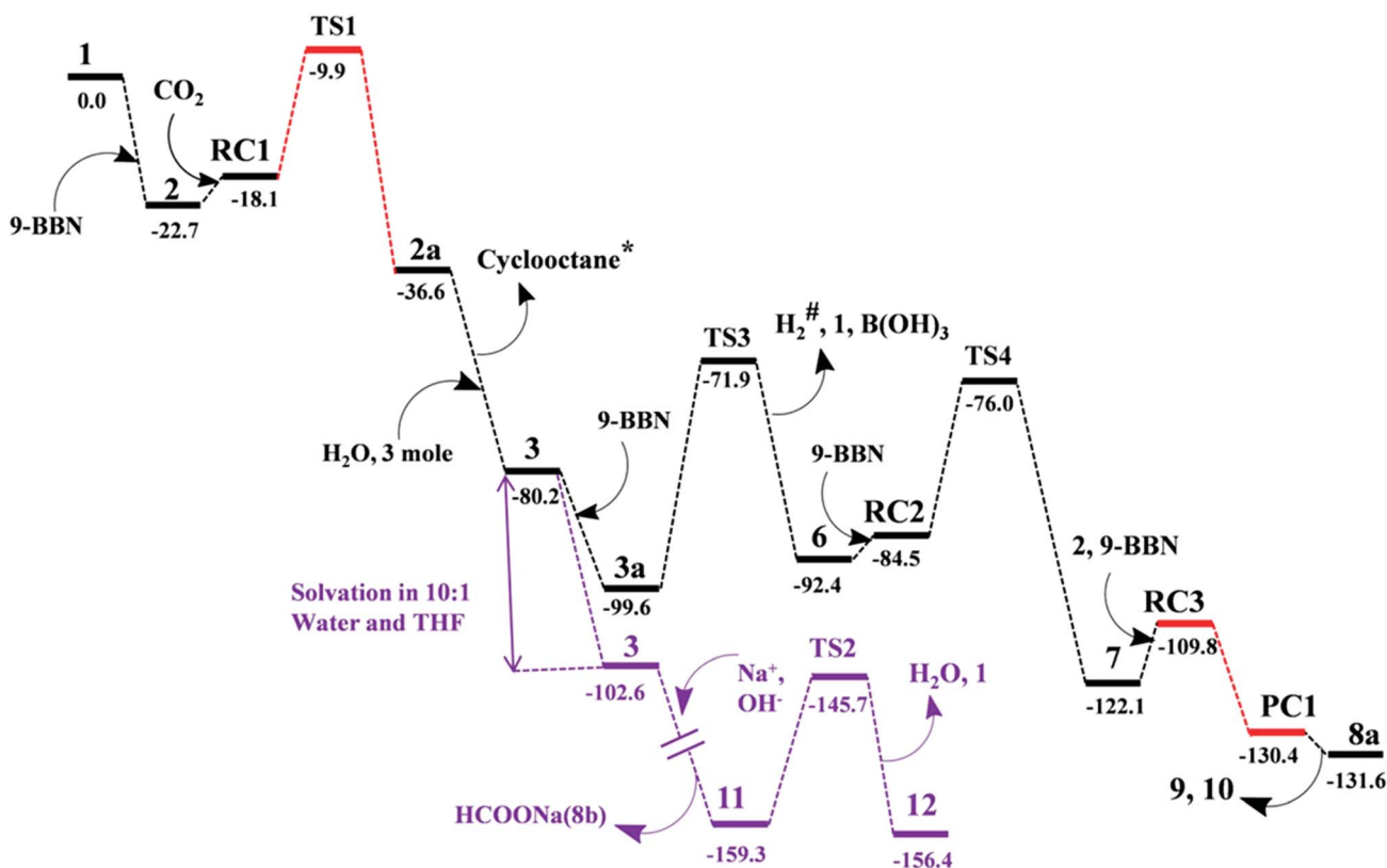
Fig. 7 Computed Gibbs free energy profiles at 25 °C for the conversion of \text{CO}_2 to methoxyborane or sodium formate with 2 in air. The relative free energies (in kcal mol -1 ) obtained in solvent were calculated with respect to the energy of the separate reactants (aNHC ( 1 ) and 9-BBN). *Formation of cyclooctane was confirmed by ^1\text{H} NMR spectroscopy. # \text{H}_2 gas evolution was confirmed by ^1\text{H} NMR spectroscopy and visual observation (see the video file in the ESI†). For drawings of all compounds see Fig. S3.†
