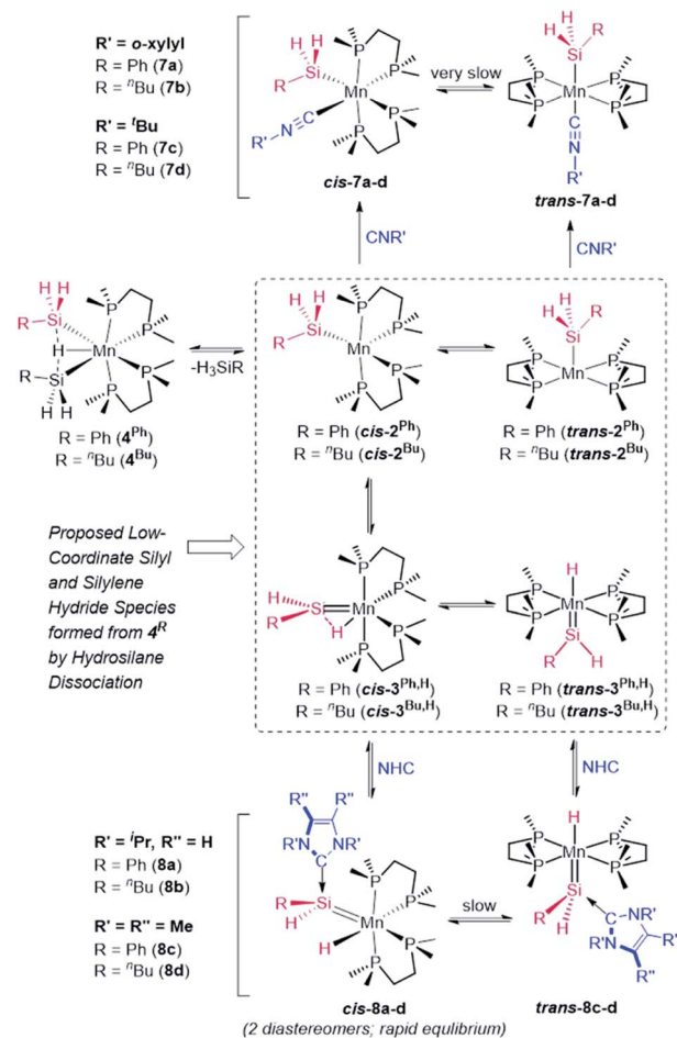
Scheme 5 Trapping of putative silyl (2 R ) and silylene hydride (3 R,H ) intermediates: synthesis of silyl isonitrile complexes [(dmpe) 2 Mn(SiH 2 R)(CNR')] (7a: \text{R} = Ph, \text{R}' = o -xylyl; 7b: \text{R} = n Bu, \text{R}' = o -xylyl; 7c: \text{R} = Ph, \text{R}' = t Bu; 7d: \text{R} = n Bu, \text{R}' = t Bu) and NHC-stabilized silylene hydride complexes [(dmpe) 2 MnH(=SiHR(NHC))] (8a: NHC = i PrNHC, \text{R} = Ph; 8b: NHC = i PrNHC, \text{R} = n Bu; 8c: NHC = Me NHC, \text{R} = Ph; 8d: NHC = Me NHC, \text{R} = n Bu).
