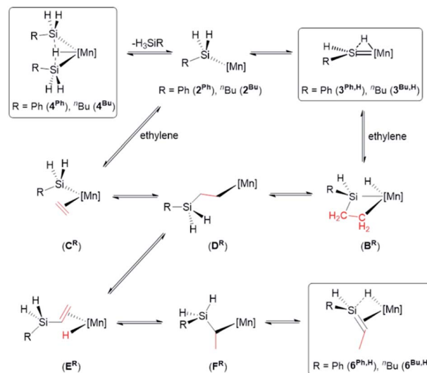
Scheme 6 Proposed pathways for reactions of disilyl hydride complexes [(dmpe) 2 MnH(SiH 2 R) 2 ] (4 R : R = Ph, 4 Bu : R = t Bu) with ethylene to form silene hydride complexes [(dmpe) 2 MnH(RHSi=CHMe)] (6 Ph,H : R = Ph, 6 Bu,H : R = t Bu). [Mn] = Mn(dmpe) 2 . Only one isomer of 3 R,H is shown. Boxes indicate complexes which have been isolated or spectroscopically observed.
