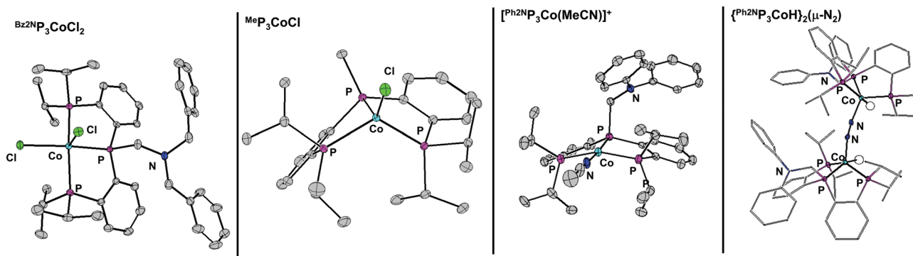
Fig. 1 50% thermal ellipsoid plot of several complexes. All hydrogen atoms not located in the difference map are removed for clarity. Only the cation of [(\text{Ph}^2\text{N}^1\text{P}_3\text{Co}(\text{MeCN}))][\text{BARF}] is shown.
