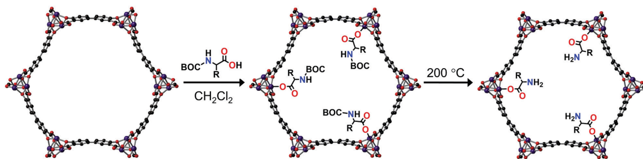
Fig. 1 Schematic of the appendage of BOC protected amino acids to the open \text{Mg}^{\text{II}} metal sites on S\text{-Mg}_2\text{dobpdc} to yield S\text{-Mg}_2\text{dobpdc}@ \text{BOC-Xxx} (Xxx = Ala, Val, Pro) where R = \text{CH}_3 (alanine), i\text{-Pr} (valine), \text{CH}_2\text{CH}_2\text{CH}_2 (proline) followed by the thermal deprotection of the BOC group to yield S\text{-Mg}_2\text{dobpdc}@ \text{Xxx} (Xxx = Ala, Val, Pro). The appendage of amino acids to 50% of \text{Mg}^{\text{II}} metal sites is shown here for clarity. The atoms are represented as follows: magnesium (purple), carbon (black), oxygen (red).
