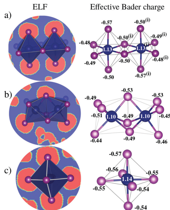
Fig. 4 Electron localization function (ELF) and effective Bader charge (e) of inorganic Bi x I y - moieties of perovskites (a) 1 , (b) 2 and (c) 3 . Along bismuth-iodide planes, the colors blue and red in the ELF plots represent electron charge depletion and accumulation, respectively.
