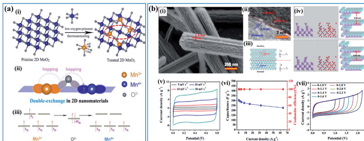
Fig. 6 (a) Double-exchange mechanism in birnessite: (i) diagram of low-oxygen-pressure thermo-annealing treatment to achieve double-exchange of \text{Mn(III)}\text{--O--Mn(IV)} in the treated birnessite nanosheet. (ii, iii) Double-exchange of \text{Mn(III)}\text{--O--Mn(IV)} results in magnetoresistance in the 2D birnessite nanosheets. 110 (b) \beta\text{-MnO}_2 /parallel birnessite core/shell nanorod: (i) SEM image of \beta\text{-MnO}_2 /parallel birnessite core/shell nanorods; (ii) high resolution TEM image of a \beta\text{-MnO}_2 /parallel birnessite core/shell nanorod (perpendicular to the 001 plane of parallel birnessite); (iii) structural representation of a \beta\text{-MnO}_2 /parallel birnessite core/shell nanorod (formation 1 and formation 2); (iv) structural computation of a \beta\text{-MnO}_2 /parallel birnessite core/shell nanorod (formation 1 and formation 2); (v) cyclic voltammograms at different scan rates (potential window: 0\text{--}0.8 \text{ V} ); (vi) variations of the capacitance and coulombic efficiency with the current densities (potential window: 0\text{--}0.8 \text{ V} ); (vii) CV curves of \beta\text{-MnO}_2 /parallel birnessite//AGO ASC at different cell voltages at a scan rate of 50 \text{ mV s}^{-1} . 49
