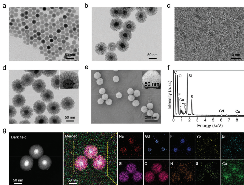
Fig. 1 Structural and compositional characterization of UMNOCC-PEG nanoparticles. TEM images of (a) the NaGdF 4 :Yb,Er core nanoparticles, (b) UCNP s @dMSN-SNO, (c) CuO 2 nanodots, and (d) UMNOCC-PEG nanoparticles. (e) SEM image and (f) corresponding EDS spectrum of the UMNOCC-PEG nanoparticles. (g) Dark-field STEM image and the corresponding elemental mappings of UMNOCC-PEG nanoparticles.
