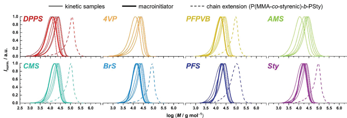
Fig. 1 Size-exclusion chromatograms obtained at various conversions during the SG1-mediated polymerization of MMA in the presence of 5 mol% of various styrenics (thin lines) at 80 °C in toluene, as well as after chain extension with styrene (dashed lines) at 120 °C in toluene from a corresponding macroinitiator (thick lines).
