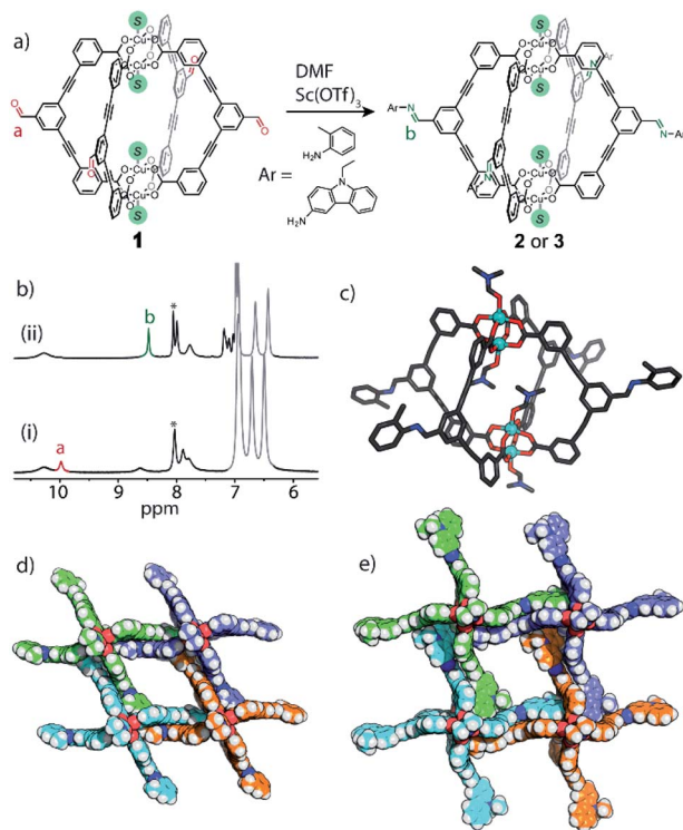
Fig. 6 (a) Scheme illustrating the covalent PAM of 1 to give 2 or 3; (b) 1 H NMR (500 MHz/DMF-d 7 ) of (ii) the reaction mixture of 2 after heating and (i) before heating. ‡ Excess aniline shown in grey. *DMF solvent peak; (c) X-ray structure of 2; (d) perspective view of the crystal packing of 2; (e) perspective view of the crystal packing of 3.
