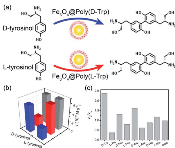
Fig. 2 (a) The enantioselective oxidation of chiral tyrosinol catalyzed by \text{Fe}_3\text{O}_4@\text{Poly(L/D-Trp)} . (b) The initial velocity for the oxidation of tyrosinol enantiomers with \text{Fe}_3\text{O}_4@\text{Poly(D-Trp)} (blue), \text{Fe}_3\text{O}_4@\text{Poly(L-Trp)} (red) and bare \text{Fe}_3\text{O}_4 (gray). (c) The ratio of initial rates for the oxidation of the D enantiomer to L enantiomer.
