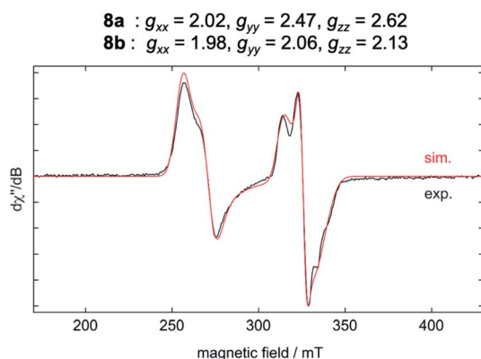
Fig. 4 EPR spectrum of 8 in the solid state at -203^\circ\text{C} with \text{NBU}_4\text{Br} .
