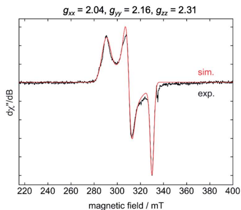
Fig. 7 Molecular structure of trans - [\text{Ni}^{\text{I}}(\text{Mes}_2\text{Im})_2(\text{C}_6\text{F}_5)] ( 11 ) (top) in the solid state (ellipsoids drawn at the 50% probability level) and EPR spectrum at -203^\circ\text{C} of the isolated compound 11 (bottom). Hydrogen atoms are omitted for clarity.
