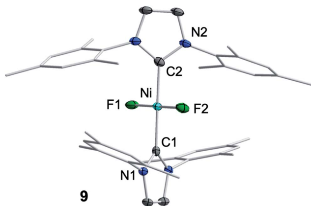
Fig. 6 Molecular structure of trans - [\text{Ni}(\text{Mes}_2\text{Im})_2(\text{F})_2] ( 9 ) in the solid state (ellipsoids drawn at the 50% probability level). Hydrogens atoms are omitted for clarity.
