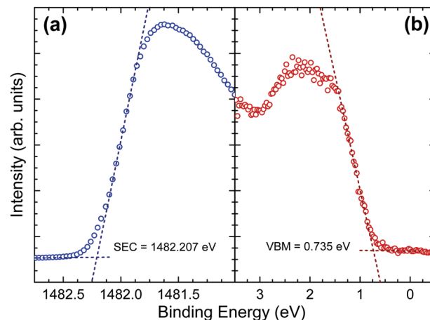
Fig. 6 (a) Secondary electron cut-off (blue) and (b) valence band maximum (red) of in situ cleaved Sb 2 Se 3 bulk crystals with straight line fits used to determine the binding energy of the cut-offs. The incident photon energy is 1486.6 eV.
