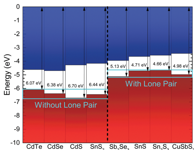
Fig. 7 Ionization potential for Sb 2 Se 3 from the photoemission results in Fig. 6, compared with literature values for other materials. 23,24,49,50 The zero of the energy scale corresponds to the vacuum level. The materials are labelled as without or with lone pair 5s 2 electrons.
