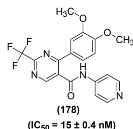
Fig. 56 Chemical structure of selected catecholpyrimidine derivative (178).
