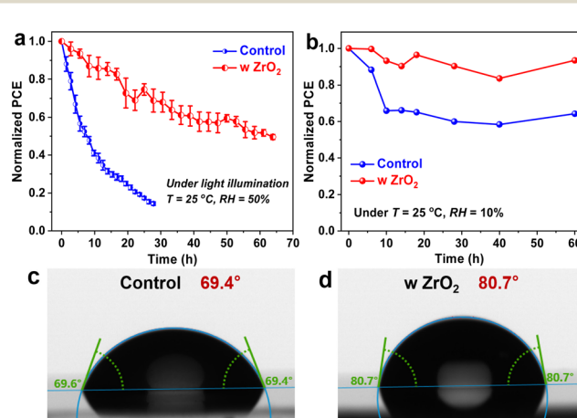
Fig. 4 (a and b) Stability levels of unencapsulated control and ZrO_2 -capped PSCs under (a) persistent light irradiation and (b) dry air conditions. The errors in the data (indicated by error bars) originate from the fluctuation of the light intensity of the xenon lamp. (c and d) Contact angles of water on perovskite films before and after they were capped with a ZrO_2 layer at T = 25 °C and RH = 50\% .
