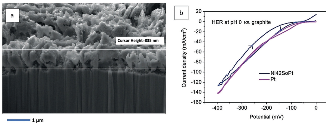
Fig. 106 (a) SEM photograph showing the cross-section of the \text{Ni}_{42}/\text{Pt} interface (Pt thickness \sim 800\text{--}900\text{ nm} ); the Pt loading is 1.8\text{ mg cm}^{-2} . (b) comparison of the HER performances of Pt and \text{Ni}_{42}\text{SoPt} at pH = 0. Reproduced with permission from ref. 1269. Copyright Wiley 2019.
