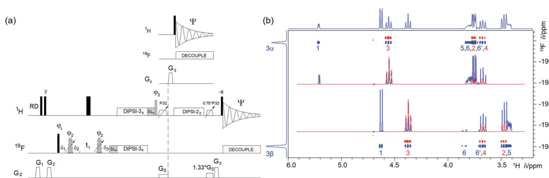
Fig. 4 (a) Pulse sequence of a 2D ^{19}\text{F} , ^1\text{H} CP-DIPS13-DIPS12. For explanation of symbols used for pulses see Experimental. The NMR parameters used are given in Table S1.† The dashed line indicates signal acquisition before an optional ^1\text{H} - ^1\text{H} spin-lock. For description of pulses see Experimental. The delays were as follows: \delta_1 = 20 \mu\text{s} ; \delta_2 = \delta_1 + (2/\pi) \times p3 ; \delta_3 = p2 ; t_1(0) is the initial t_1 evolution delay time = 0.5 \times \text{in}0 , where \text{in}0 is the t_1 increment. The gradient strengths were as follows: G_0 = 5\% ; G_1 = 17\% ; G_2 = 31\% ; G_3 = 66\% . The following phase cycling was used: \varphi_1 = y, -y ; \varphi_2 = 4x, 4(-x) ; \varphi_3 = 2y, 2(-y) ; \Psi = x, 2(-x), x . The states-TPPI protocol was used for sign discrimination in F_1 with the phase \varphi_1 incremented by 90^\circ . Purging of ^{19}\text{F} magnetisation at the beginning of the pulse sequence by a composite 90^\circ ^{19}\text{F} pulse and PFGs minimises the cancellation artefacts. (b) An overlay of two 2D ^{19}\text{F} , ^1\text{H} CP-DIPS13-DIPS12 spectra acquired with 20 ms ^{19}\text{F} \rightarrow ^1\text{H} cross-polarisation (CP) only (red) and an additional 50 ms ^1\text{H} \rightarrow ^1\text{H} spin-lock (blue) using the pulse sequence shown in (a). The red spectrum was offset vertically to facilitate visualisation of the cross peaks. The two insets show overlaid 1D F2 traces through ^{19}\text{F} resonances of \alpha - and \beta -D-glucose from both spectra. Twice as many scans were acquired for the blue spectrum as for the red spectrum. 1D ^{19}\text{F} and ^1\text{H} projections of the blue spectrum are shown along the left and top, respectively.
