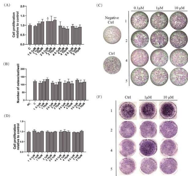
Fig. 3 The osteoblastogenesis and osteoclastogenesis activities of compounds 1 , 2 , 4 , and 5 . (A) Cell proliferation activity of RAW264.7 cells; (B) quantitative of osteoclasts (TRAP positive multi-nucleated cells (MNCs), more than 3 nuclei) induced from RAW264.7 cells by osteoclast differentiation medium for 4 days ( n = 3 ). (C) Representative images of TRAP staining osteoclast at day 4 in each well of 96-well plate. (D) Cell proliferation activity of pre-osteoblast MC3T3-E1 cells; (E) representative morphological pictures of ALP staining on the MC3T3-E1 cells induced by osteoblast differentiation medium at day 6. NC: negative control, 0.1% DMSO without osteoclast differentiation medium (OCM); C: control, 0.1% DMSO with OCM; results were obtained from three independent experiments in triplicate and expressed are means \pm SD; * P < 0.05 , ** P < 0.01 , *** P < 0.001 significantly different from the control group.
