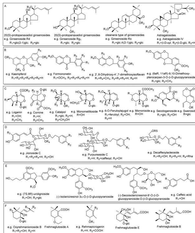
Fig. 4 The main structure types of compounds identified in this work: saponins (A), flavonoids (B), iridoids (C), phenylethanoid glycosides (D), phenylpropanoids (E), and ionones (F).
