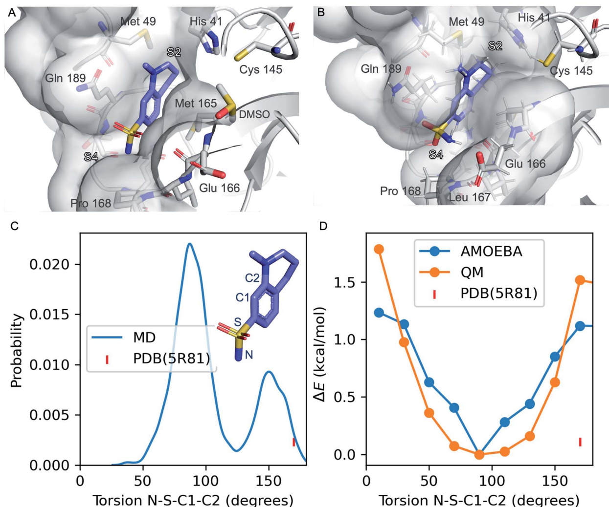
Fig. 1 Refinement of the co-crystal structure of x0195 and M^{\text{pro}} using MD simulations. (A) An unusual conformation of x0195 (in purple) located in the binding pocket formed by His41, Met49, Glu166, Gln189, and Pro168 and their surroundings (PDB code: 5R81), and (B) the relaxed structure of x0195 (in purple), obtained after the equilibration step, interacting with the amino acid residues of the substrate binding site. M^{\text{pro}} is shown in light grey. (C) Torsion angle distribution for the sulfonamide group during 20 ns of MD simulations (in blue) performed on the M^{\text{pro}} dimer in complex with x0195; the torsion angle of the sulfonamide group in the co-crystal structure is shown in pink. (D) Torsion energy scan calculated by AMOEBA (in blue) and QM (in orange); the torsion angle of the sulfonamide group in the co-crystal structure is shown in pink. QM level = \omega\text{B97x-D/6-31g}^{*65-67} .
