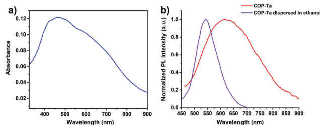
Fig. 2 (a) The UV absorption spectrum of COP-Ta in the solid state. (b) Fluorescence spectra of COP-Ta in the solid state (red) and dispersed in ethanol (purple), respectively ( \lambda_{ex} = 365 nm).
