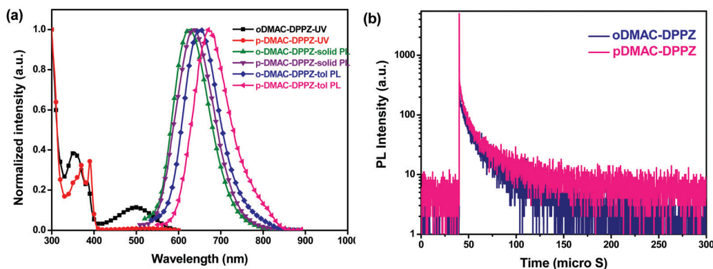
Fig. 2 (a) UV-vis absorption and PL spectra of oDMAC-DPPZ and pDMAC-DPPZ TADF emitters in toluene and those of 1% TADF-emitter-doped PS films at room temperature. (b) Transient PL decay curves of 1 wt% oDMAC-DPPZ - and pDMAC-DPPZ -doped thin PS films acquired at 300 K under a nitrogen atmosphere.
