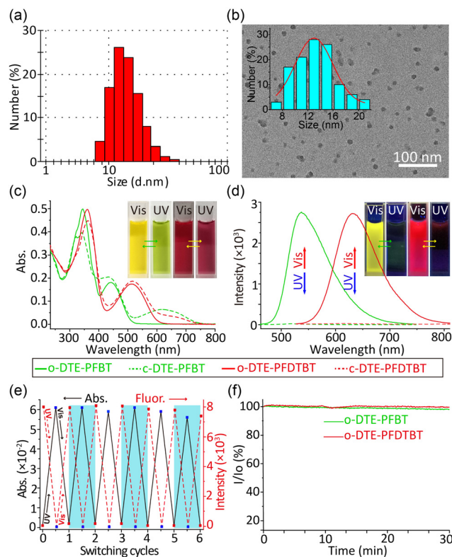
Fig. 1 Particle size and morphology of DTE-PFBT Pdts measured by DLS (a) and TEM (b). (c) The absorption and (d) fluorescence spectra of Pdts solutions under 365 nm ( 2 \text{ mW cm}^{-2} ) and 620 nm ( 50 \text{ mW cm}^{-2} ) irradiation. Insets: Pictures of the colour and fluorescence changes upon light irradiation. (e) Absorbance (620 nm) and corresponding fluorescence (536 nm) changes of DTE-PFBT Pdts during repetitive and alternate irradiation. (f) Photostability of Pdts under continuous excitation. I/I_0 is the ratio of the fluorescence intensity under irradiation to the initial fluorescence intensity.
