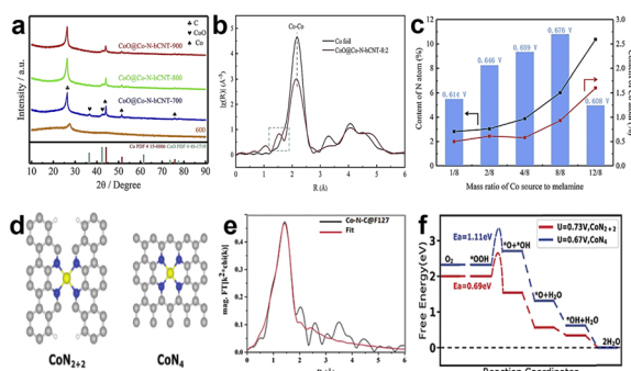
Fig. 10 (a) XRD patterns of \text{CoO@Co-N-bCNT} samples synthesized at different temperatures. 80 (b) Co K-edge EXAFS spectra of \text{CoO@Co-N-bCNT-8:2} (8:2 is mass ratio of Co source to melamine) and Co foil. 80 (c) Relationship among E_{1/2} , N content and Co content of the \text{CoO@Co-N-bCNT} samples. 80 (d) Structure of \text{CoN}_{2+2} and \text{CoN}_4 active sites. 84 (e) The fitted spectra of FT-EXAFS for the Co–N–C@F127 catalyst. 84 (f) Free energy evolution diagram for the 4e^- ORR pathway on the \text{CoN}_{2+2} and \text{CoN}_4 active sites. 84
