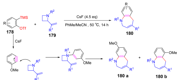
Scheme 25 2-Vinylazetidines with benzyne of the [6 + 2] cycloaddition reaction.
