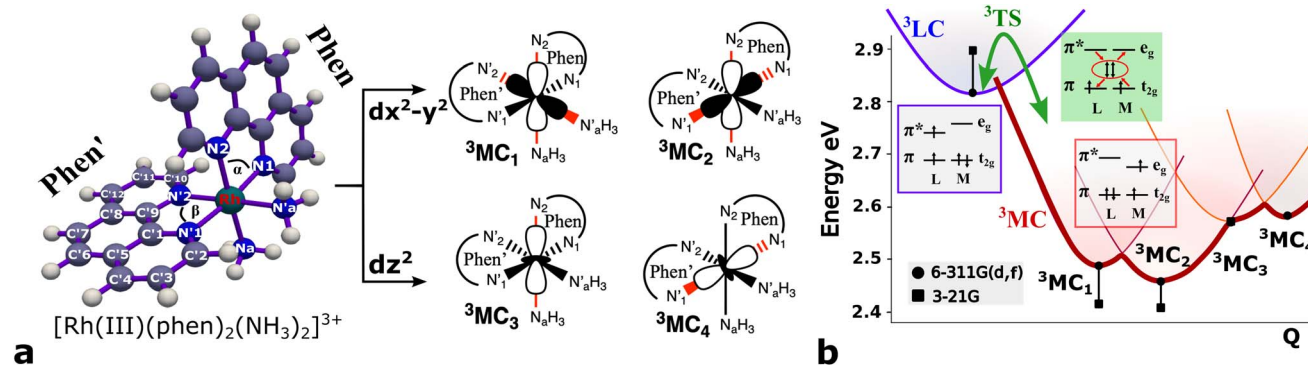
Fig. 1 Chemical structure and triplet excited state properties of the [\text{Rh(III)(phen)}_2(\text{NH}_3)_2]^{3+} complex. (a) Chemical structure with key labels and e_g metal orbital orientations in [\text{Rh(III)(phen)}_2(\text{NH}_3)_2]^{3+} metal complex. (b) Triplet excited state energies (black) for the ^3\text{LC} and ^3\text{MC} states. The energy is referenced to the ground state energy in eV. Dots designate B3LYP*/6-311G(d,f)/PCM(water), and squares designate B3LYP*/3-21G/PCM(water) results. The calculated energies are combined with a schematic description of the conversion between ^3\text{LC} and ^3\text{MC} states.
