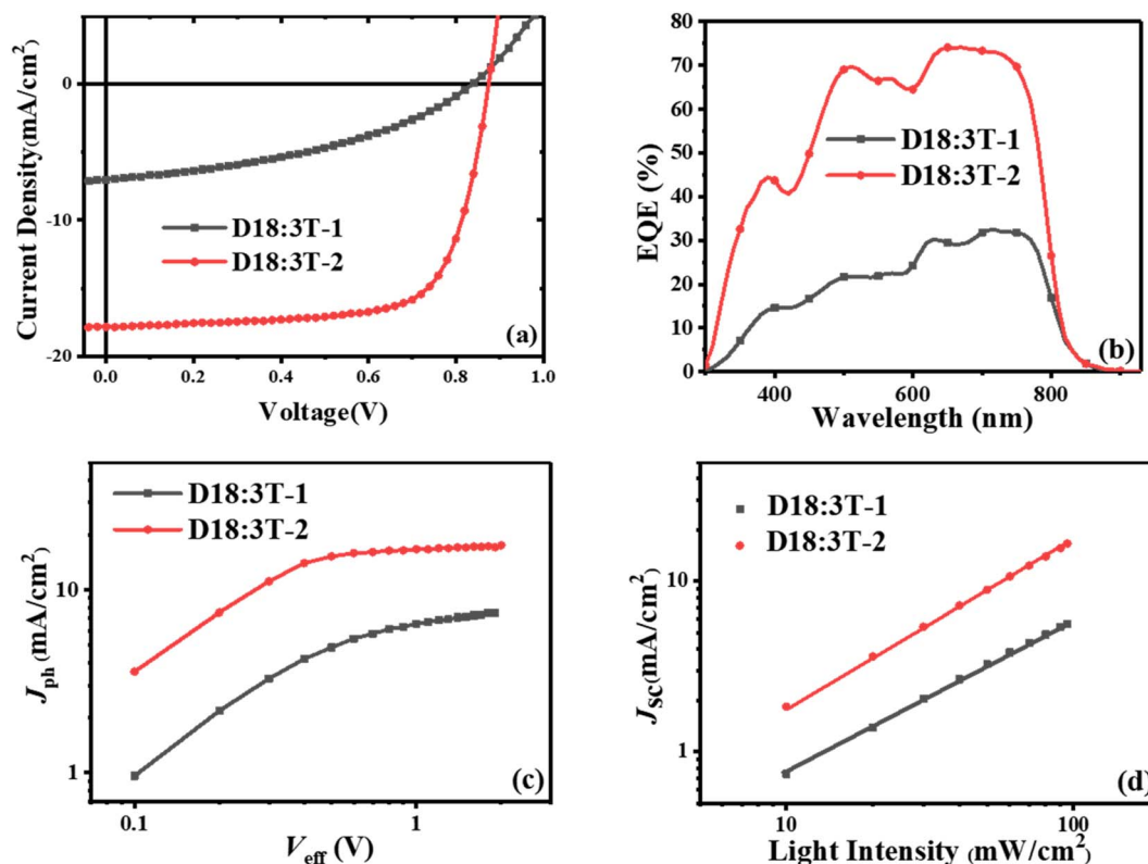
Fig. 2 (a) J-V curves and (b) EQE curves, (c) photocurrent versus effective voltage ( J_{\text{ph}}-V_{\text{eff}} ) characteristics and (d) light intensity dependence of the optimized 3T-1 and 3T-2 based devices.
