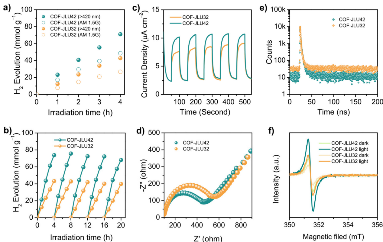
Fig. 6 (a) Photocatalytic hydrogen evolution activity of COF-JLUs under visible-light irradiation ( \lambda > 420\text{ nm} ) and AM 1.5G (5 mg of COF-JLU in 50 mL of H 2 O, 3 wt% Pt as a cocatalyst, 0.1 M AA as SED). (b) Photocatalytic stability of COF-JLUs (5 mg of COF-JLU in 50 mL of H 2 O, 3 wt% Pt as a cocatalyst, 0.1 M AA as SED, \lambda > 420\text{ nm} ). (c) Transition photocurrents of COF-JLUs under visible-light illumination. (d) EIS spectra of COF-JLUs. (e) Time-resolved PL spectra of COF-JLUs. (f) EPR spectra of COF-JLUs in the dark and under visible-light illumination.
