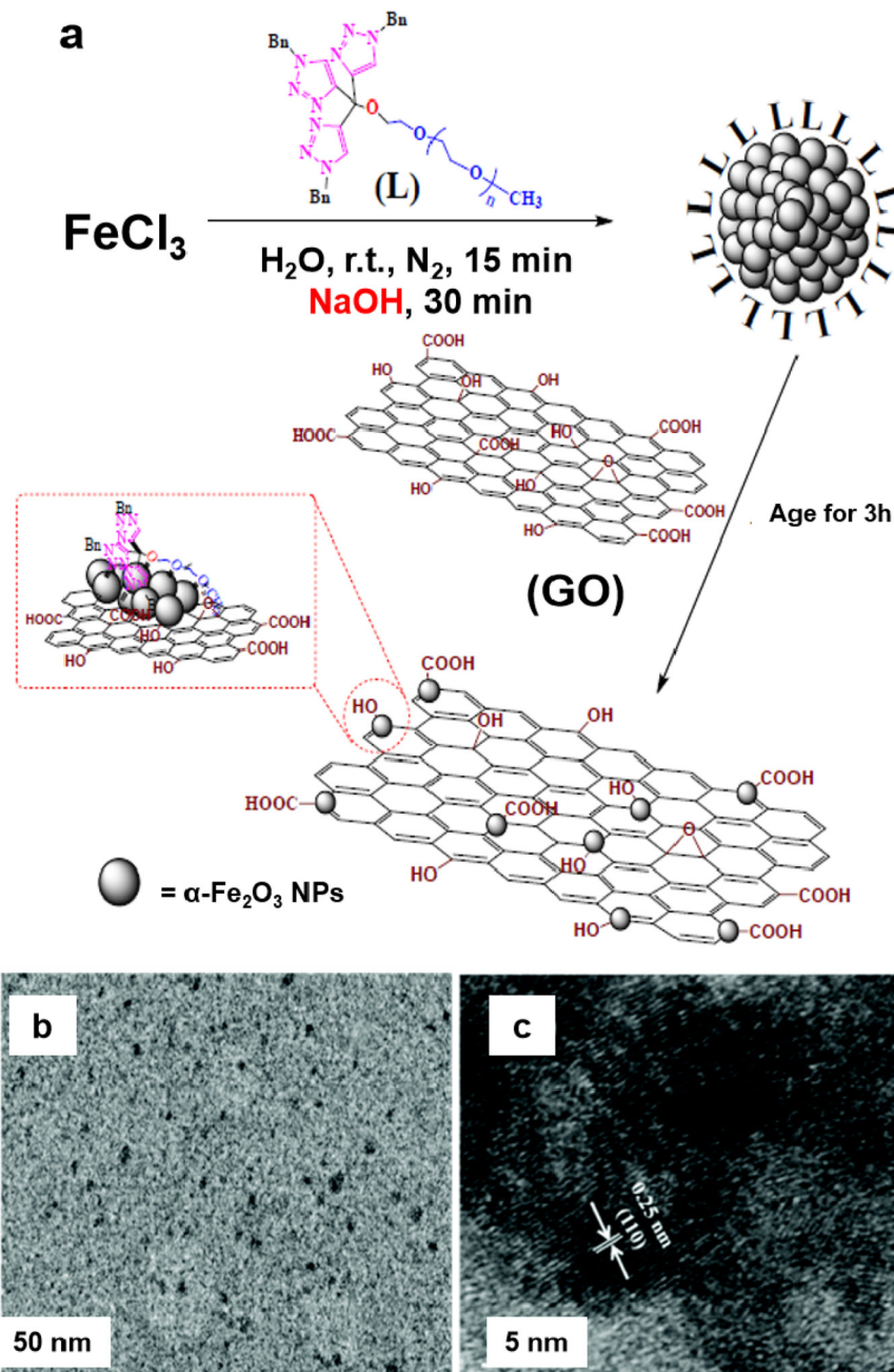
Fig. 8 (a) Schematic representation for the synthesis of the \alpha\text{-Fe}_2\text{O}_3/\text{GO} catalyst; (b, c) TEM and HR-TEM images of \alpha\text{-Fe}_2\text{O}_3 nanocluster/GO catalyst. Reproduced with permission from ref. 135 Copyright 2017, The Royal Society of Chemistry.
