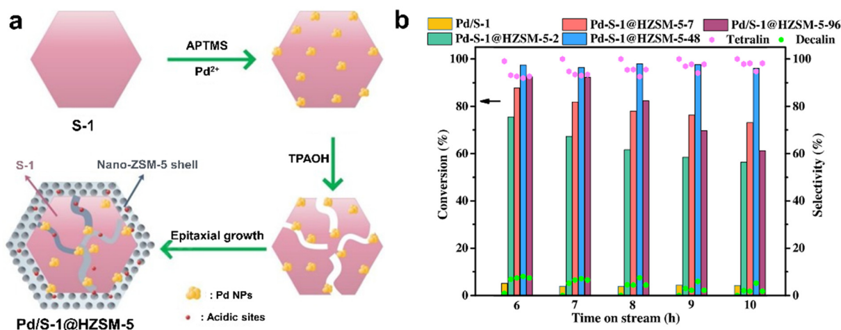
Fig. 14 (a) The preparation progress for the \text{Pd/S-1@HZSM-5} catalyst; (b) catalytic performances of naphthalene hydrogenation over different catalysts (reaction conditions: WHSV = 1.3 \text{h}^{-1} , \text{H}_2/\text{feed} = 750, 4 MPa \text{H}_2 , 280 °C). 118 Reprinted with permission from Elsevier B.V., copyright 2021.
