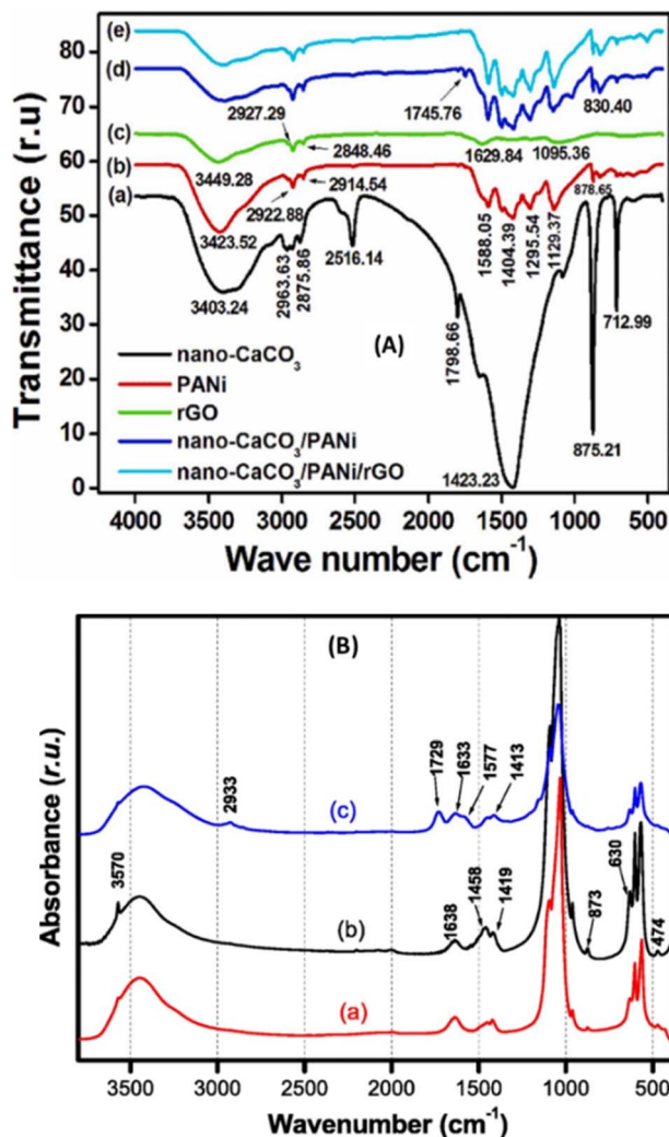
Fig. 2 (A) FTIR spectra of (a) nano- \text{CaCO}_3 , (b) PANi, (c) rGO, (d) nano- \text{CaCO}_3 /PANi, and (e) nano- \text{CaCO}_3 /PANi/rGO. This figure has been reproduced from ref. 23 with permission from Elsevier Ltd., copyright 2022. (B) FTIR spectra of (a) NHAP, (b) NHAPP0.5, and (c) NHAPP0.5-CA- \beta -CD materials. This figure has been reproduced from ref. 40 with permission from Springer-Verlag GmbH Germany, copyright 2021.
