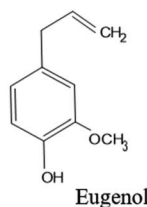
Fig. 5 Chemical structures of several compounds, assigned to different groups, present in EOs, including terpenes (e.g., monoterpenes and sesquiterpenes), terpenoids, and aromatic compounds.
