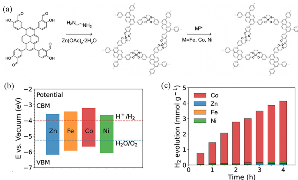
Fig. 30 (a) Synthesis and structure of Zn-Salen-COF and M/Zn-Salen-COF ( \text{M} = \text{Fe}, \text{Co}, \text{Ni} ). (b) Schematic energy band structures of Zn-Salen-COF and M/Zn-Salen-COF. (c) Photocatalytic \text{H}_2 production on Zn-Salen-COF and M/Zn-Salen-COF. Reproduced with permission. 99 Copyright 2023, Wiley-VCH GmbH.
