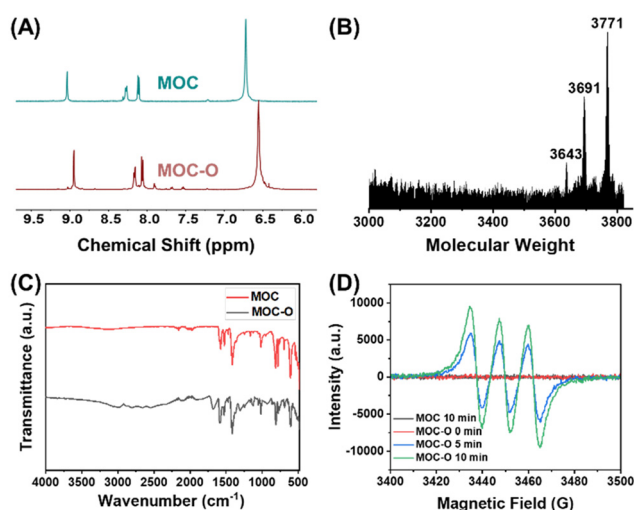
Fig. 1 The structural characterization of MOC and MOC-O nanozymes. (A) The ^1\text{H-NMR} spectra of the MOC and MOC-O in \text{DMOS-}d_6 . (B) The MALDI-TOF mass spectrum of the MOC-O. (C) The FT-IR spectra of the MOC and MOC-O. (D) The EPR curves of the MOC and MOC-O.
